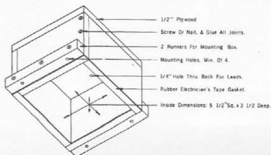
Figure 2 - Diagram of recommended inner enclosure
