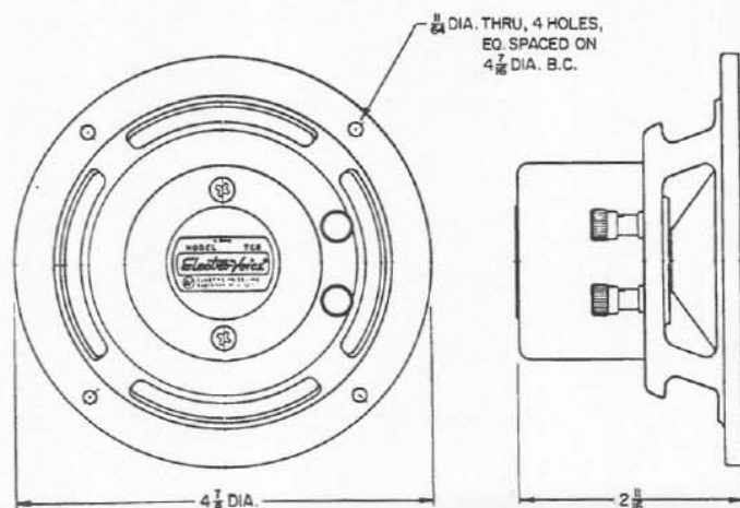
Figure 1 - Dimensions
